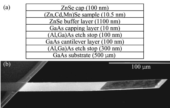
FIG. 1. (a) Schematic of the MBE-grown heterostructure. The 10.5-nm-thick magnetic layer is grown as a digital alloy (seven iterations of: 1/16th monolayer of MnSe followed by 4 15/16th monolayer of \text{Zn}_{0.87}\text{Cd}_{0.13}\text{Se} ). The etch stop layers are grown as a random alloy ( \text{Al}_{0.7}\text{Ga}_{0.3}\text{As} ). (b) SEM photo of a 100-nm-thick, 250\ \mu\text{m} long cantilever supporting a rectangular mesa of paramagnetic (Zn,Cd,Mn)Se.
