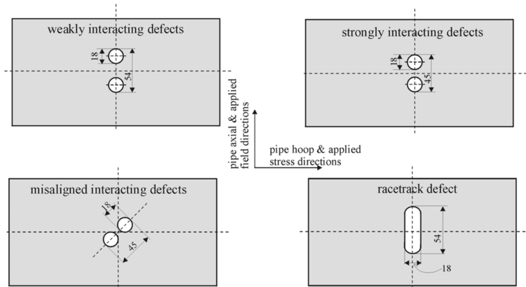
Fig. 2. Defect geometries investigated. All dimensions are given in mm
